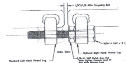
Bolt Ring Closure
